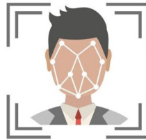
FACE RECOGNITION
